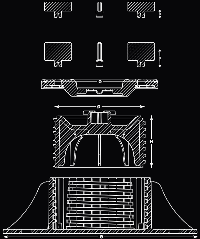
COMPOSIZIONE BASAMENTI REGOLABILI SPECIAL MF / COMPOSITION OF ADJUSTABLE SUPPORTS SPECIAL MF / COMPOSICIÓN SOPORTES REGULABLES SPECIAL MF
